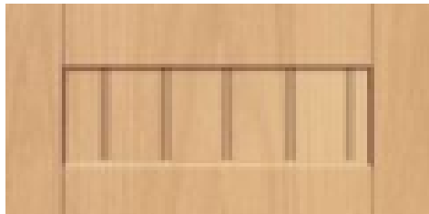
Mortise & Tenon Drawer #10 3/4" Thick Mortise & Tenon Construction with 1/4" Flat Veneer Center Panel with 1 1/2" spaced beads
